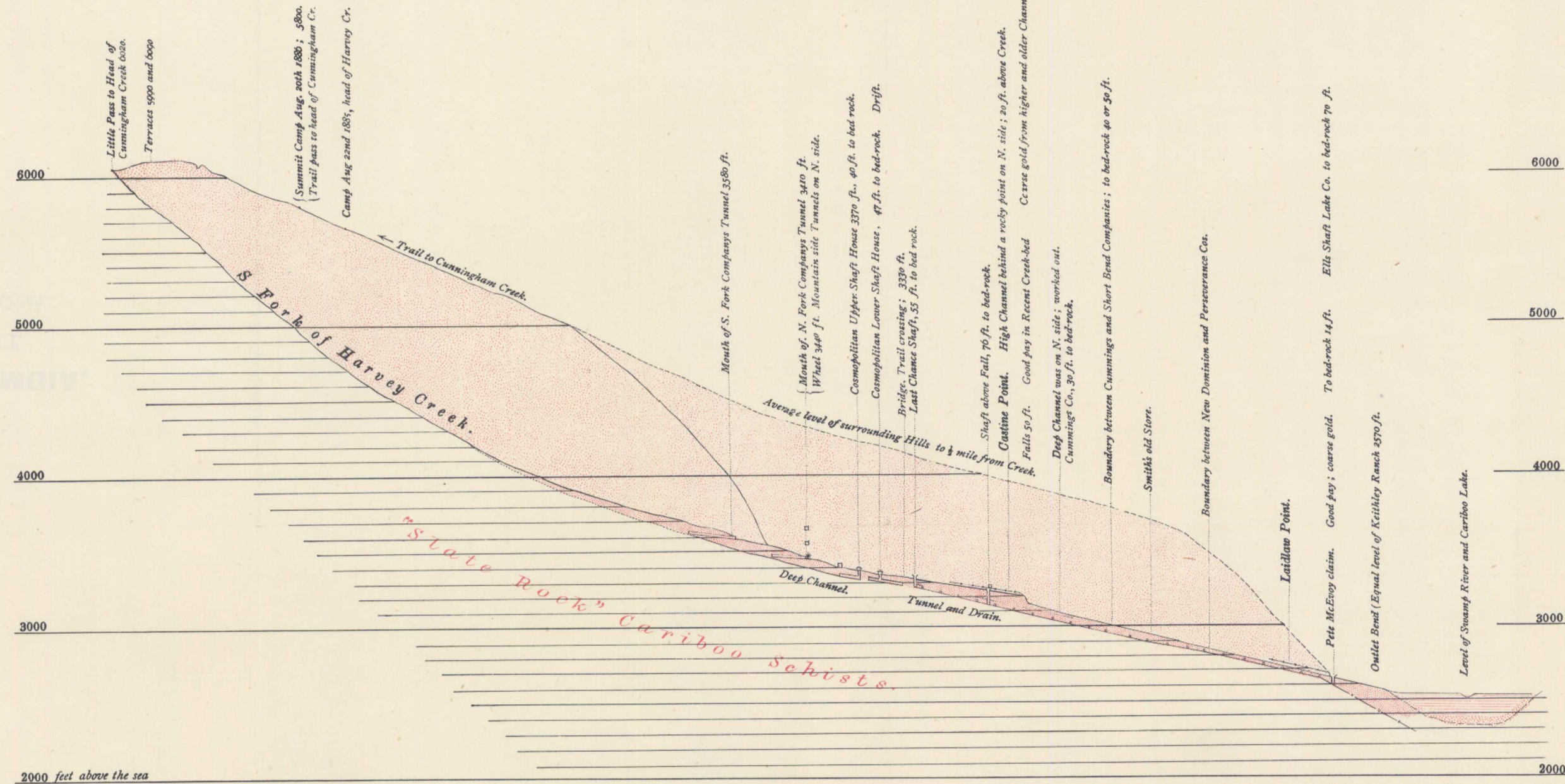
SECTION ALONG HARVEY CR Showing explorations of Deep Channel Vertical Scale exaggerated 5 times to 1 of Horizontal distance.
